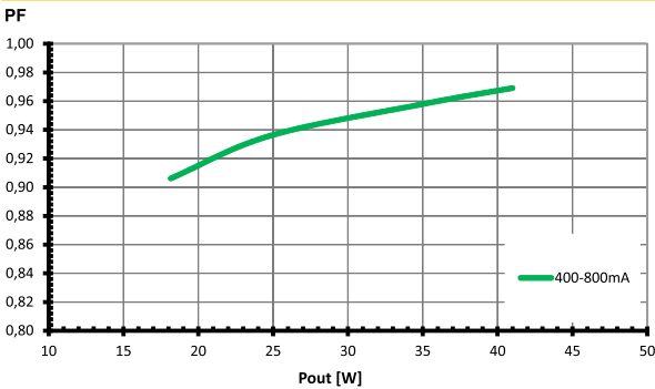
Power factor
