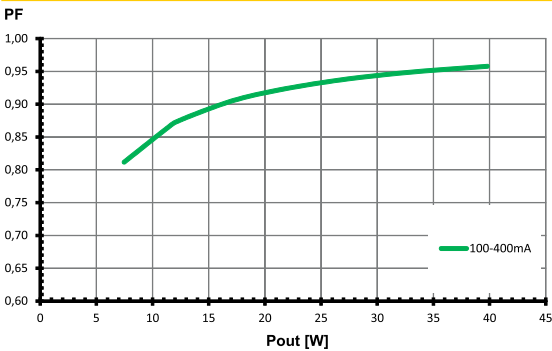
Power factor
