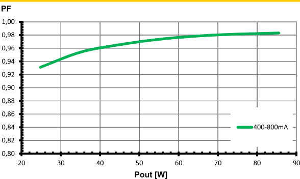
Power factor
